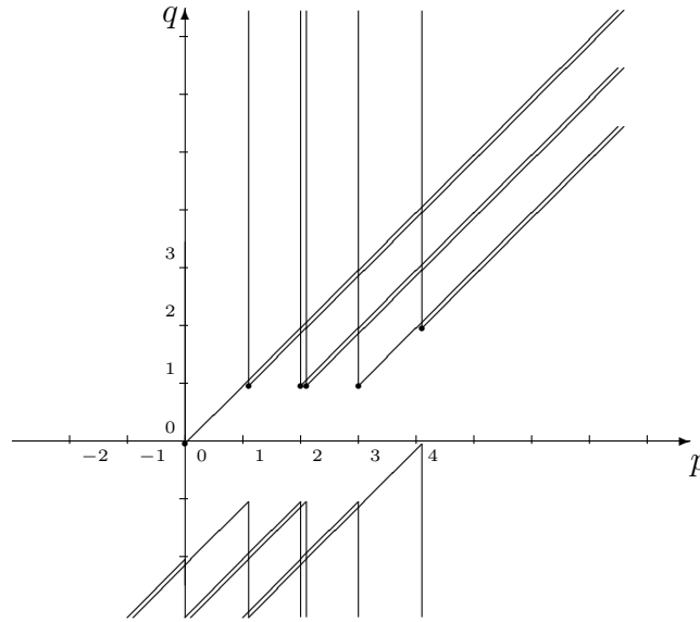
Fig. VIII.2: The E_1 term of the spectral sequence of the filtration of G_2(\mathbb{R}^{4,1}) with \varphi_2 = (3) .
