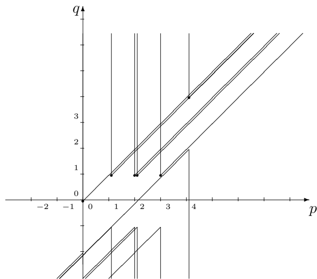
Fig. VIII.6: The E_1 page of the cellular spectral sequence for G_2(\mathbb{R}^{4,2}) using \varphi_3 = (3, 4) .
