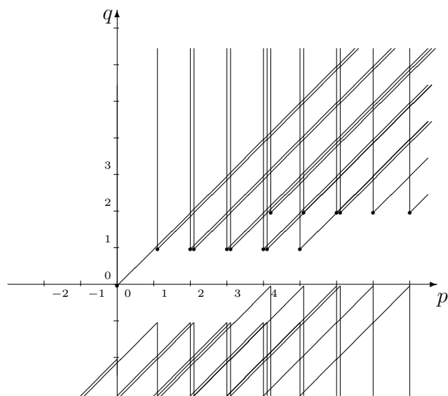
Fig. VIII.10: H^{*,*}(G_2(\mathbb{R}^{6,1}))
