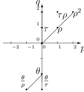
Fig. II.1: H^{*,*}(pt; \mathbb{Z}/2)
