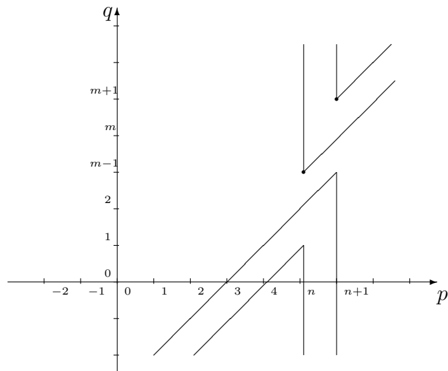
Fig. VII.3: The E_1 page of the cellular spectral sequence for \mathbb{R}P^n for n even using flag symbol (1, 2, \dots, a-1, n+1) .
