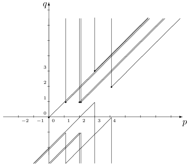
Fig. VIII.5: The E_1 page of the cellular spectral sequence for G_2(\mathbb{R}^{4,2}) using \varphi_2 = (2, 4) .
