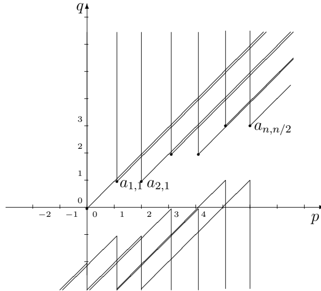
Fig. VII.2: The E_1 page of the cellular spectral sequence for \mathbb{R}P^n for n even.
