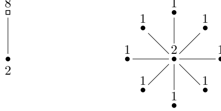
FIGURE 4. Left: The quiver defining the nilpotent orbit X in the case n = 8 . Right: The star quiver Q_n^{\text{star}} , with dimension vector \mathbf{v}'' , defining X // T , also for n = 8 .
