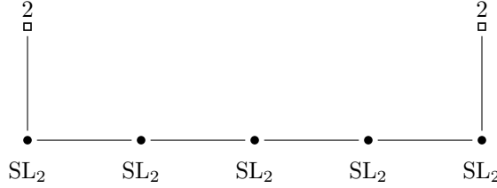
FIGURE 5. The variety \mathcal{M}_C , for n = 8 , as a Hamiltonian reduction of the form (T^* \text{Hom}(\mathbb{C}^2, \mathbb{C}^2))^6 // (\text{SL}_2)^5 .
