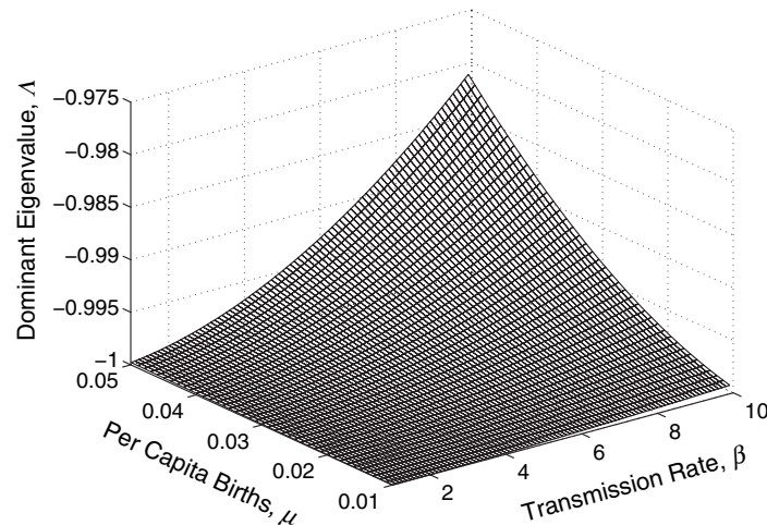
Figure 2.12. The stability of the endemic equilibrium for the SIR model phrased in discrete-time. The magnitude of the dominant eigenvalue is always less than one, but not massively so, suggesting very weakly stable dynamics; the dominant eigenvalue is also real and negative, indicating a 2-week oscillatory cycle in the approach to equilibrium.
