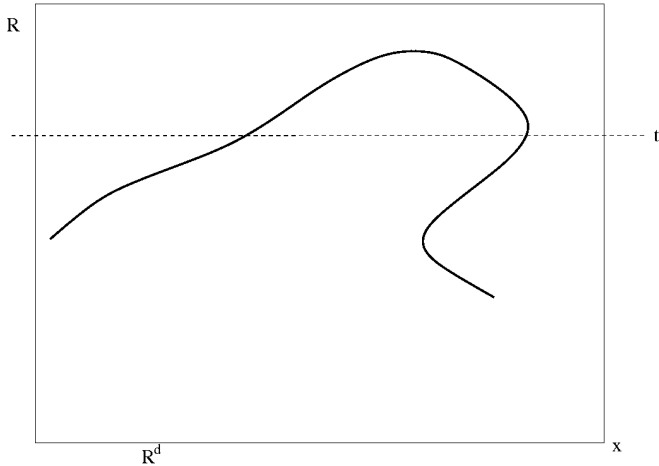
Figure: The (x, t) variables in the lemma
