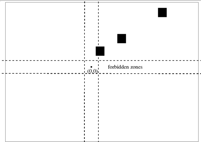
Figure: The type of chain arising in the elimination of (E, x) and \underline{\omega}
