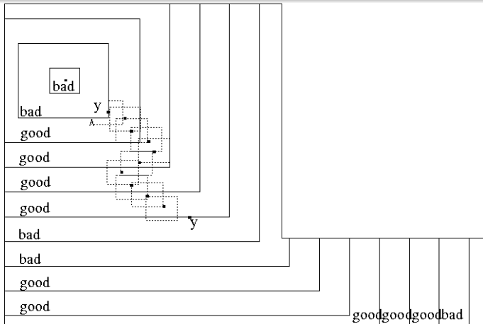
Figure: Applying the resolvent identity with good and bad cubes
