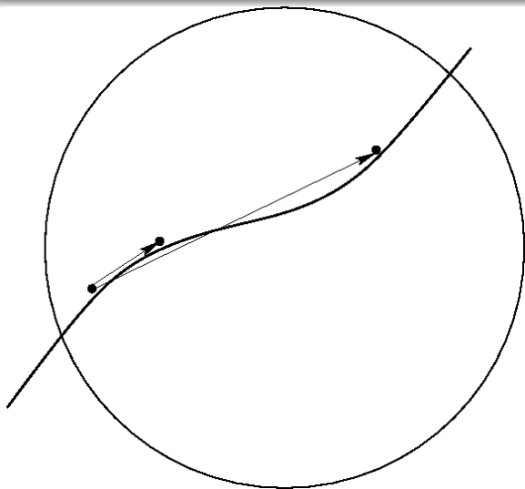
Figure: The geometry in the proposition
