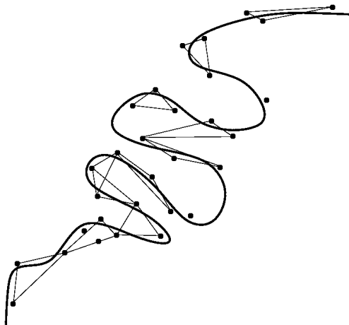
Figure: Curve, points, triangles
