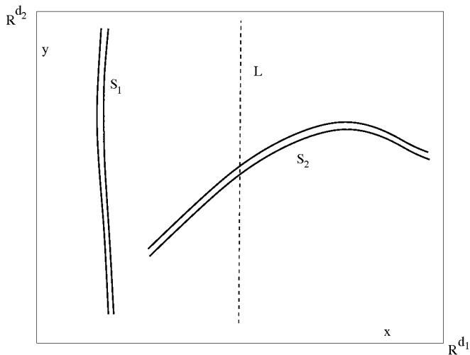
Figure: The sets S_1 and S_2
