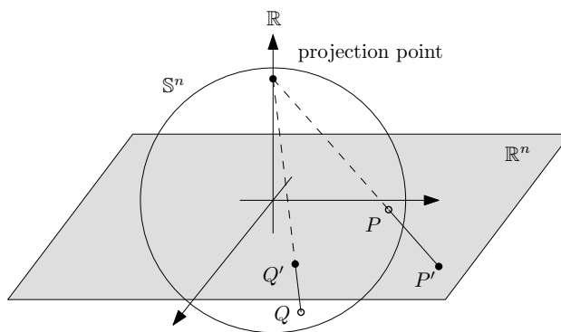
FIGURE 7. Stereographic projection of \mathbb{S}^n
