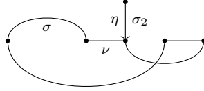
FIGURE 3. Steenrod module structure of the 20-skeleton of B ; the bottom cell (in dimension 0) is on the left; straight lines are \mathrm{Sq}^4 , and curved lines correspond to \mathrm{Sq}^8 and \mathrm{Sq}^{16} , in order of increasing length. The bottom two attaching maps of B are labeled. The map \sigma_2 is shown.
