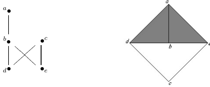
Fig. 1: A finite space and its associated simplicial complex.
