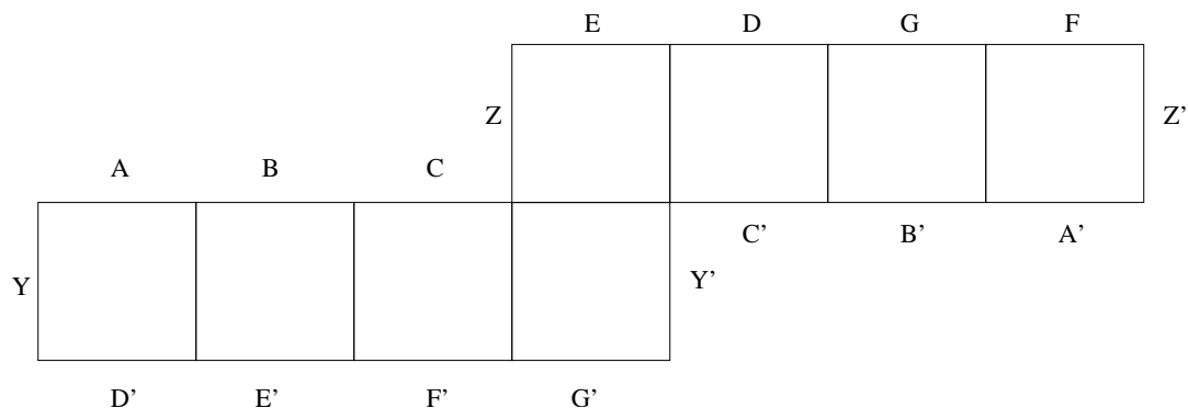
Figure 2.1: A square-tiled surface with \text{SL}(X, \omega) = \text{SL}(2, \mathbb{Z}) .
