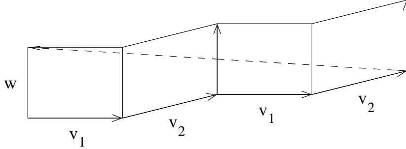
Figure 2: \beta_-^{-2} as a single saddle connection.
