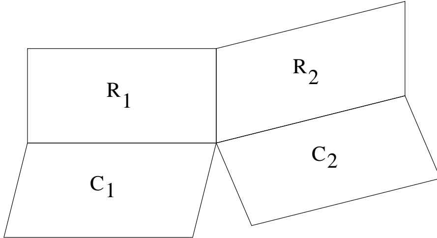
Figure 1: Normal form for (X, \omega) .
